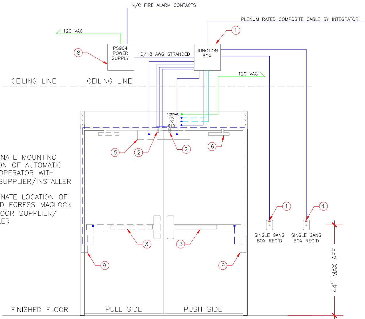
DOOR ELEVATION NOT TO SCALE
