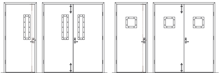
PN(F) Narrow and PV(F) Vision Lights – LM 9300
