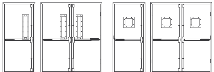
ADA Compliant PN(F) Narrow and PN(F) Vision Lights – WS98/9927, WS98/9957
