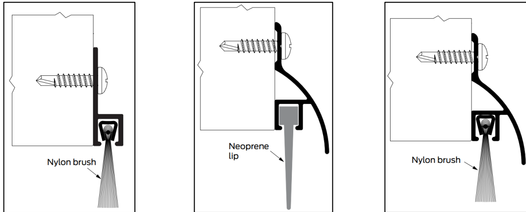
Figure 2: Zero Door Sweeps (Left to Right: 8192AA, 8197AA, 8198AA)
