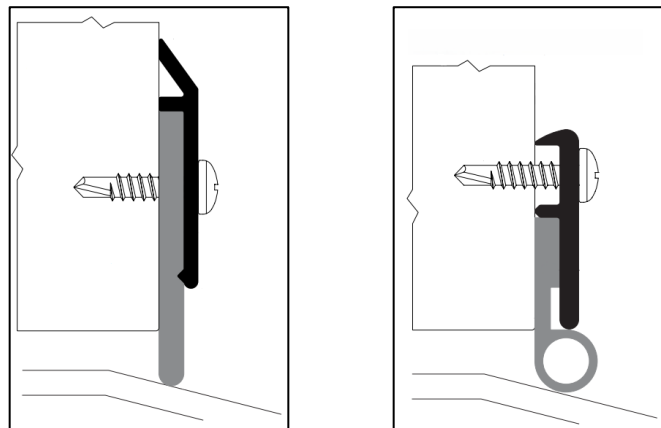
Figure 1: Zero Door Sweeps (Left to Right: 39AA, 328AA)
