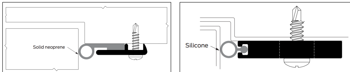
Figure 1: Zero Head and Jamb Gasketing (Left to Right: 328AA, 429AA)
