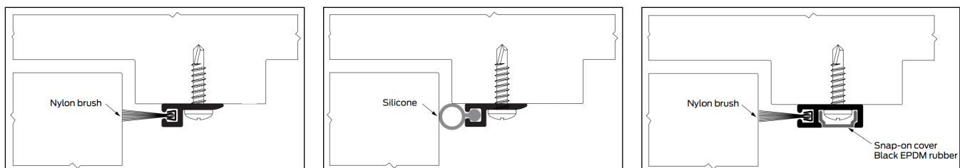
Figure 2: Zero Head and Jamb Gasketing (Left to Right: 8193AA, 8303AA, 8879AA),
