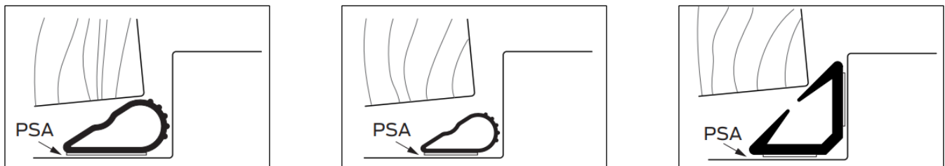
Figure 1: Zero Weatherstripping (Left to Right: 188S, 488S, 8144S)
